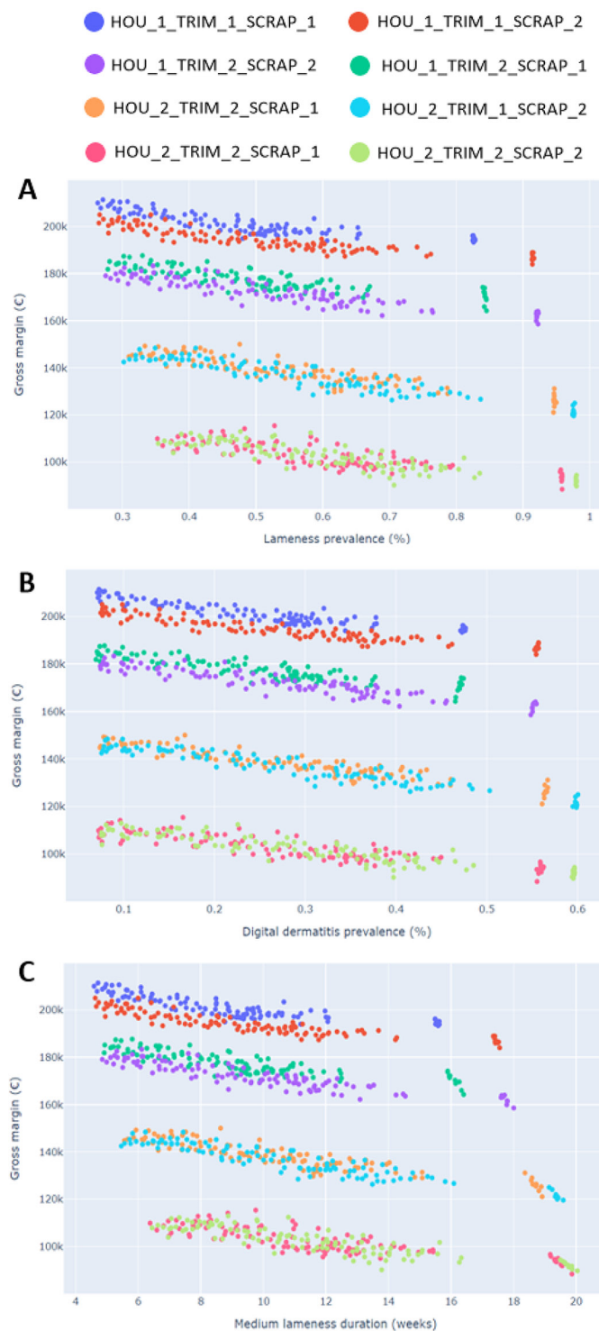
Figure 4. Relationship between gross margin and the different combinations of scenarios for (A) lameness, (B) digital dermatitis, and (C) medium lameness duration. HOU_1 = concrete floor; HOU_2 = textured floor; TRIM_1 = preventive trimming; TRIM_2 = no preventive trimming; SCRAP_1 = scraping frequency >8 times/d; SCRAP_2 = scraping frequency \leq 8 times/d.
